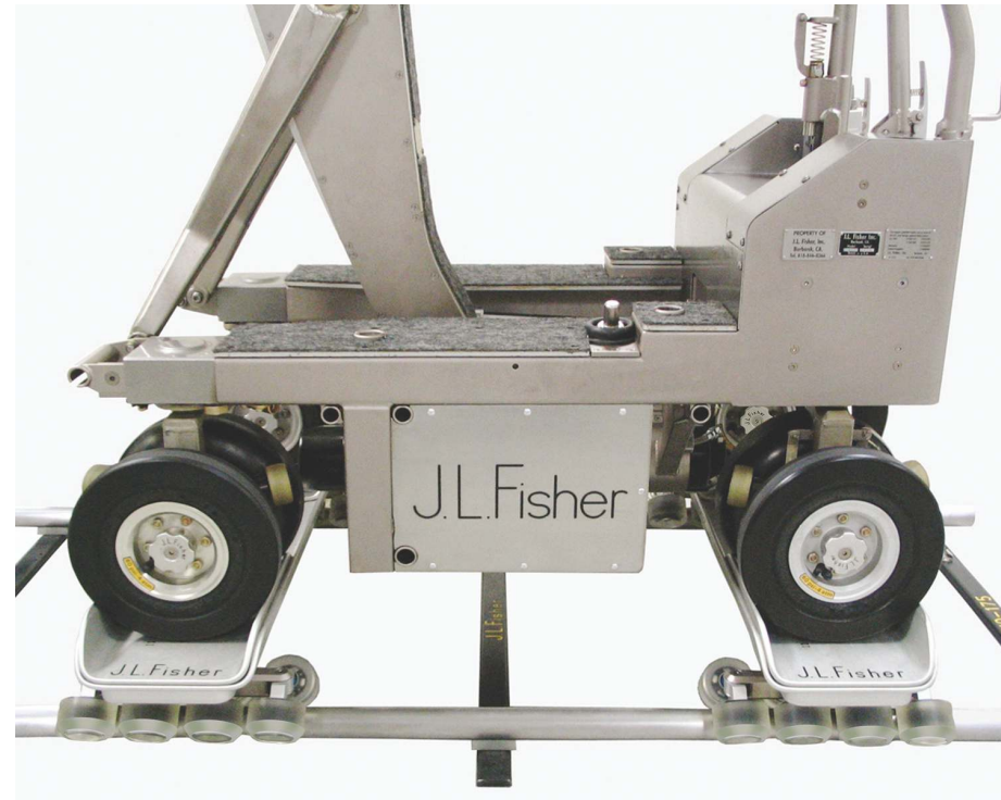
11 Dolly - mounted on standard 24.5 inch track (With insert trays)
