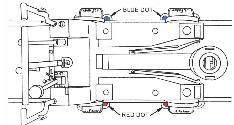
Note: When placing the skate board wheels onto the track, the red dots on the trucks must be on one side of the track, and the blue dots on the other side of the track.
